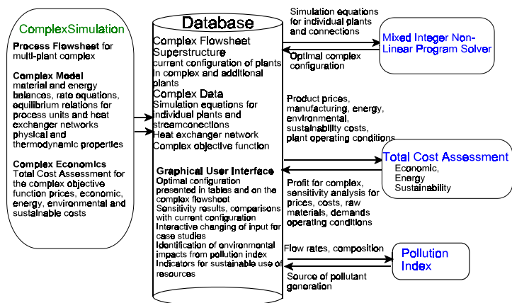
Figure 3 Program Structure for the Chemical Complex Analysis System
